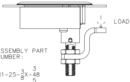
SHORT PAWL
